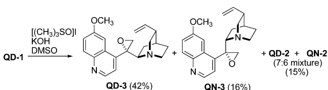
Scheme 2. Reaction of Dimethylsulfoxonium Methylide
