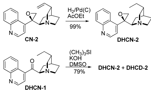
Scheme 6. Synthesis of 10,11-Dihydroepoxides
