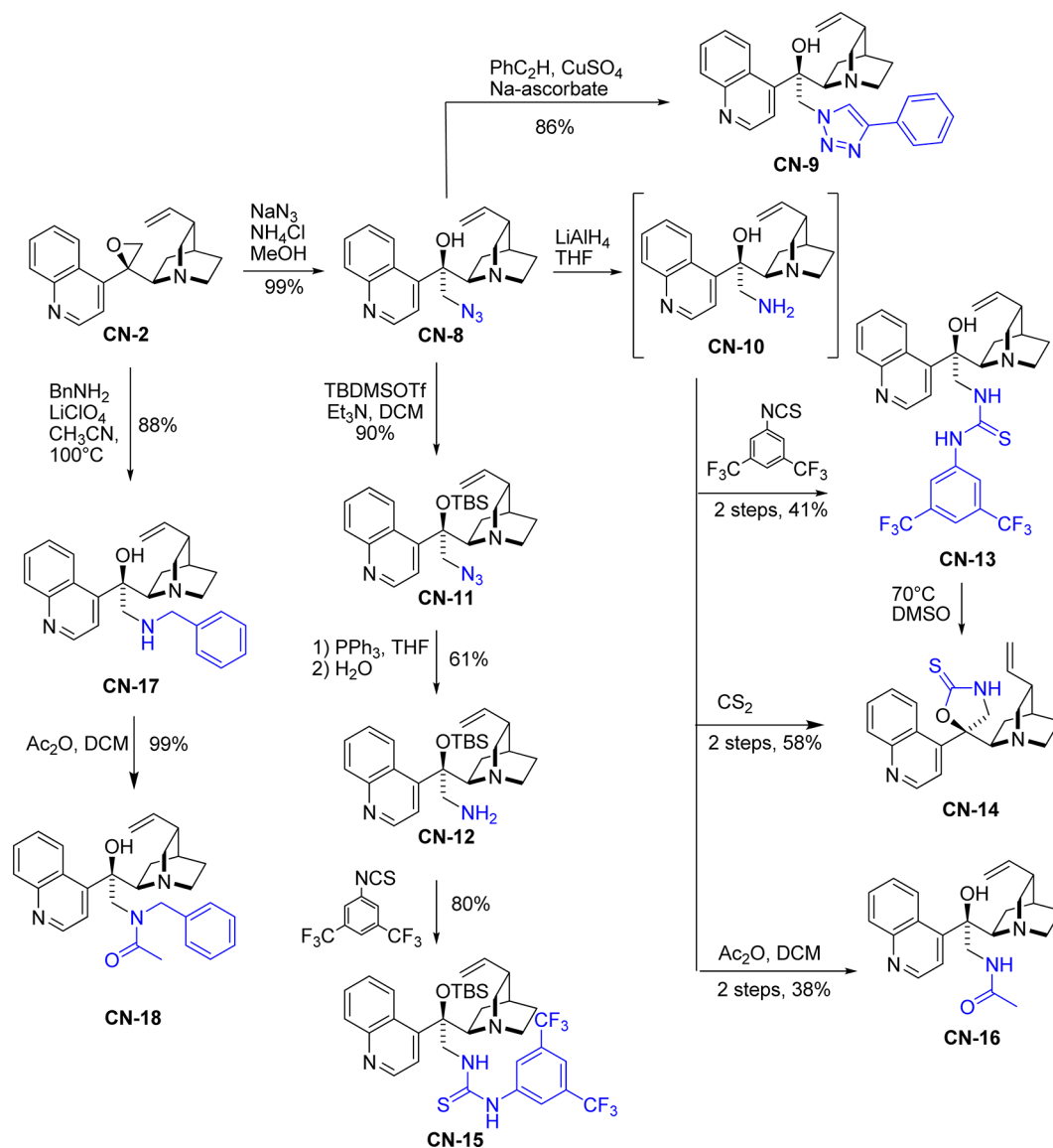
Scheme 6. Synthesis of 10,11-Dihydroepoxides
