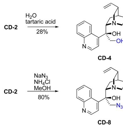
Scheme 7. Selected Reactions of Epoxide CD-2
