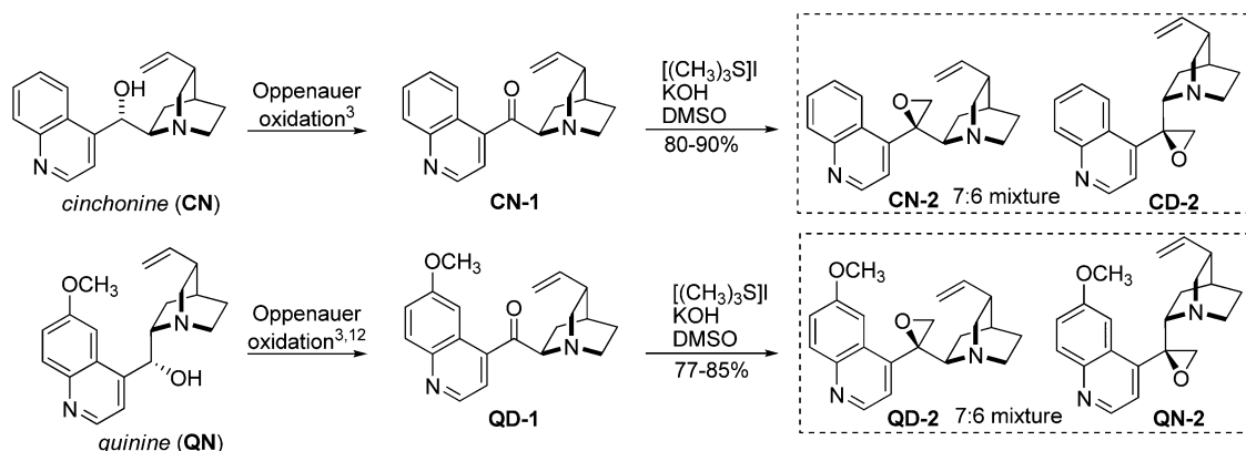
Scheme 2. Reaction of Dimethylsulfoxonium Methylide
