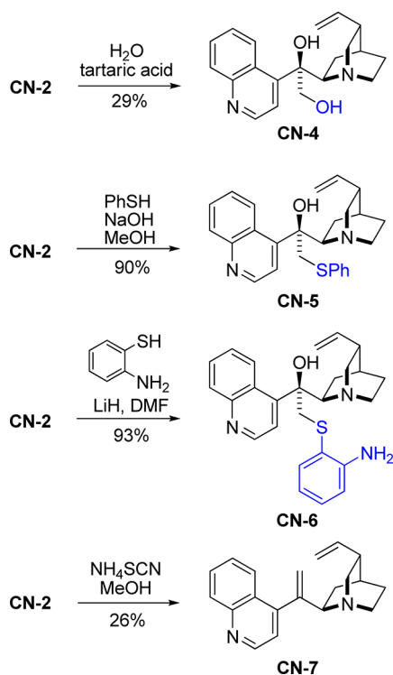
Scheme 4. Reaction of Epoxide CN-2 with Chalcogen Nucleophiles
