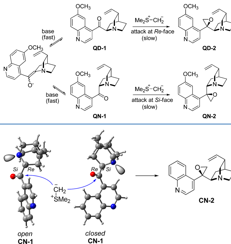
Figure 3. DFT/B3LYP/6-31G(d,p) low energy conformations and reactivity of CN-1. Re and Si faces of carbonyl group are marked.
